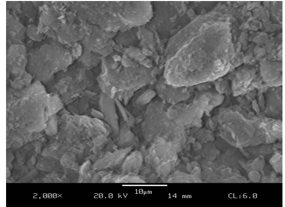
High-Resolution SEM of the Graphite Used in OCL Regular™
